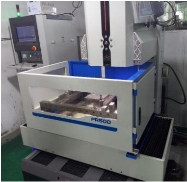
Low speed WEDM
